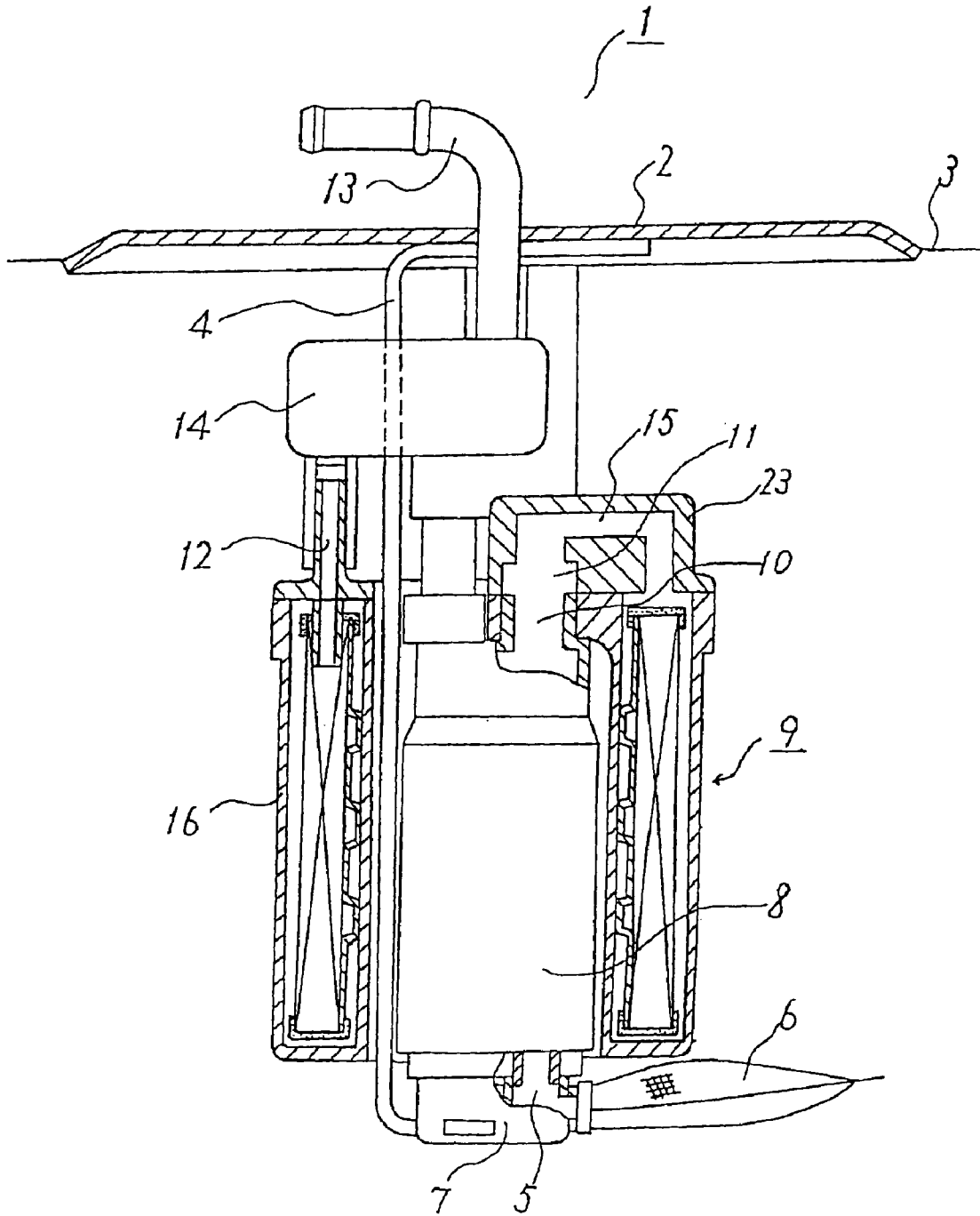
Fig. 9 (PRIOR ART)
